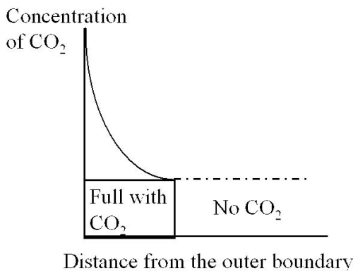
Figure 1. Complete separation of reactants in the carbonation process. The task is to predict the depth at which \text{CO}_2 is able to penetrate until a given time t \in S_T .
