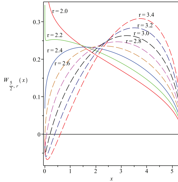
Figure 2: As in Fig. 1 for Raney distributions W_{5/2,r}(x) .
