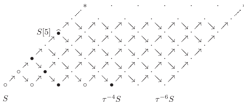
FIGURE 4.1. Lemma 4.9 (2) with r = 6 , \bullet = a branch B , \hat{\bullet} = its root, * = Prüfer summand of T ; \circ = undercut B^> as in (4.9)
