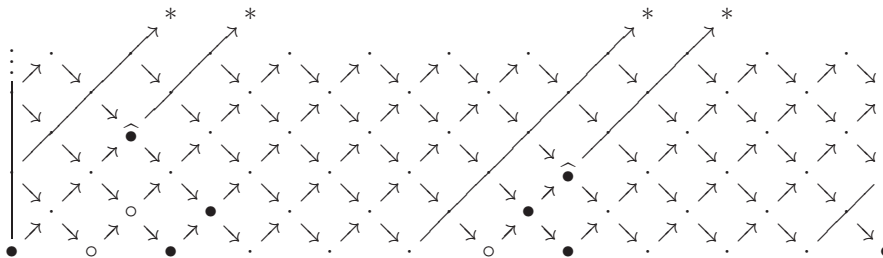
FIGURE 10.1. The branches of Example 10.7
