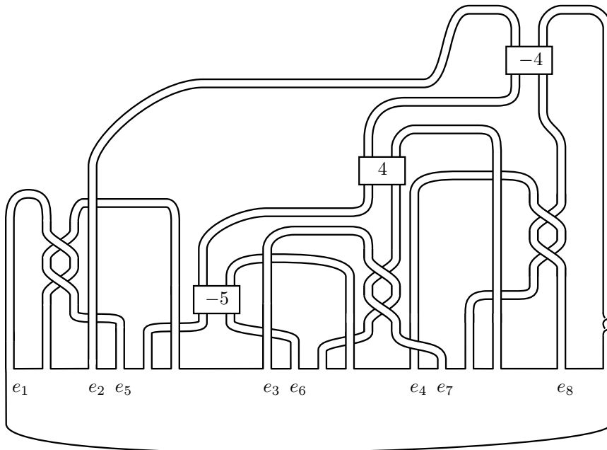
FIGURE 1. Realisation of the Seifert form V .
