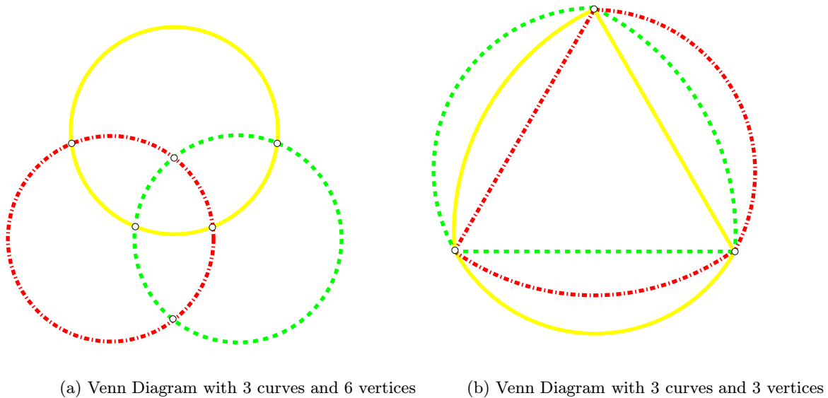
Figure 1: Example of a simple and a non-simple 3-Venn diagram.
