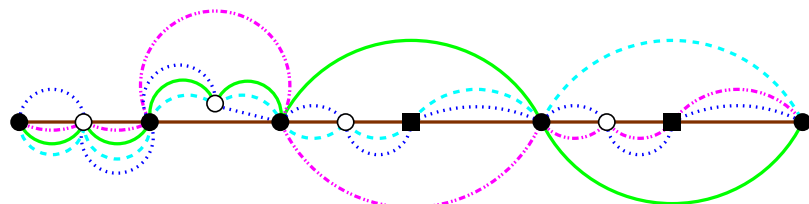
(c) Compression of vertices along the new curve.
