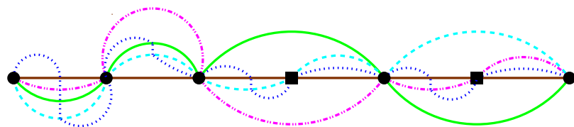
(b) The new curve moving through V_4 .
