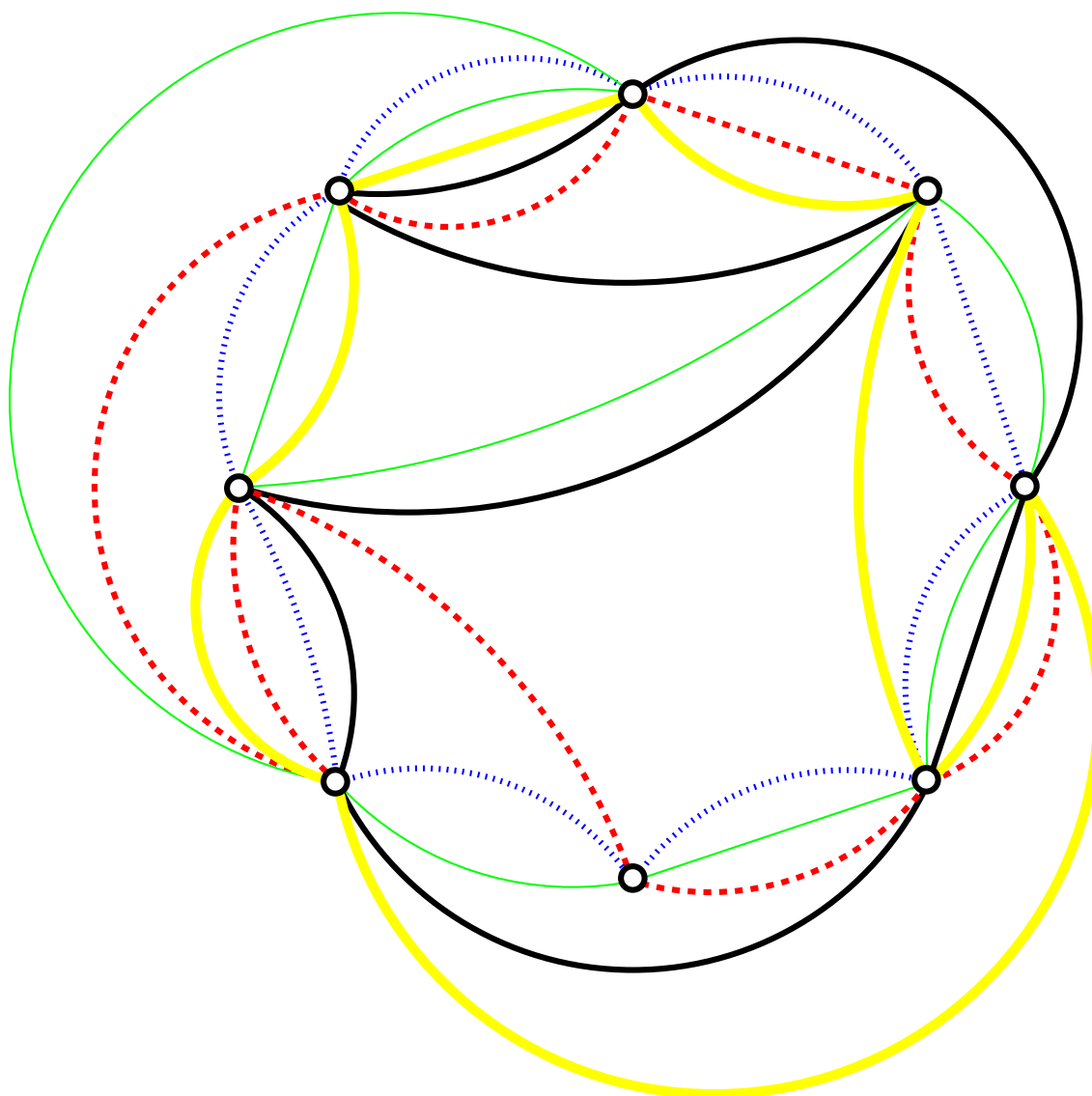
Figure 4: A 5-Venn diagram with 8 vertices.
