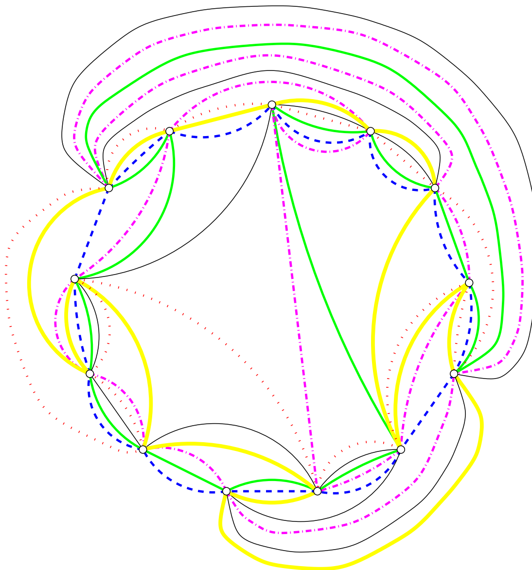
Figure 5: A 6-Venn diagram with 13 vertices.
