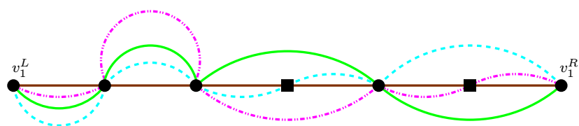
(a) The diagram V_4 .
