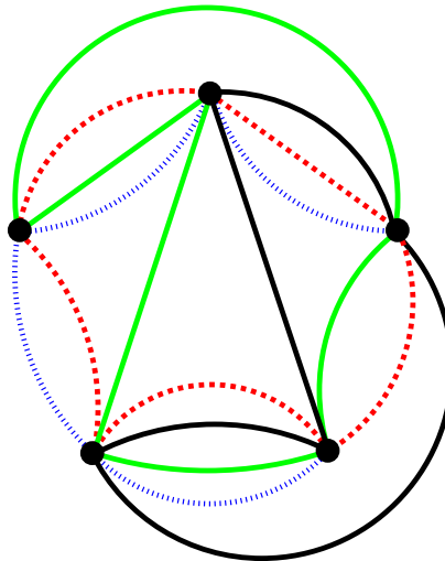
Figure 3: A 4-Venn diagram with 5 vertices.
