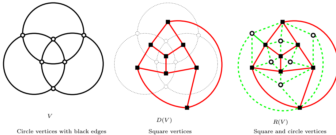
Figure 2: The radual graph construction.
