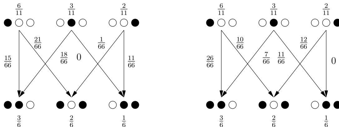
Figure 2: The two extreme solutions to the coupling problem for n = 4 and k = 2, 3 (as drawn in Figure 1). The arrows are labelled with the joint probabilities \mathbb{P}(B^k = b, B^{k+1} = b') .
