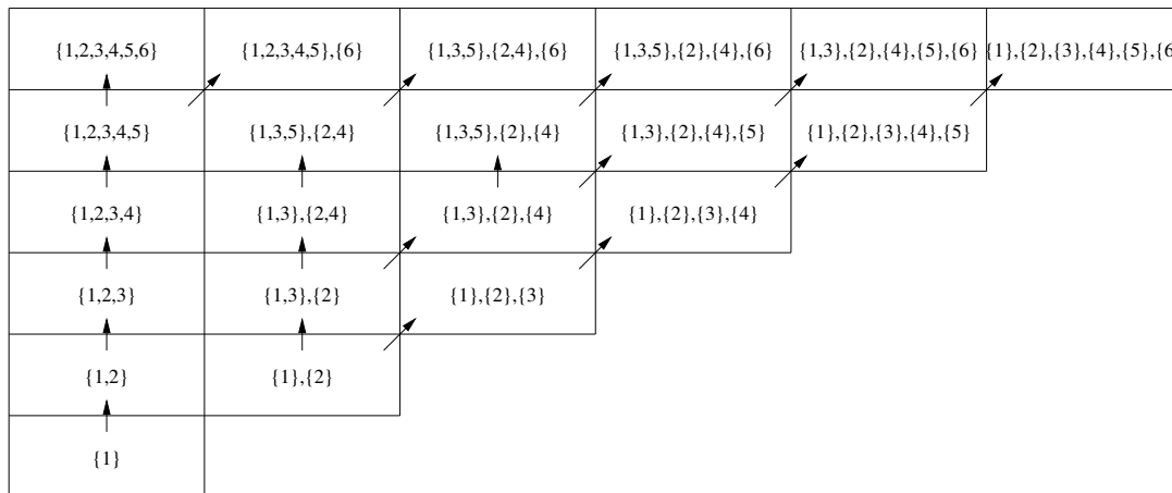
Figure 3: A possible realisation of the coupling.
