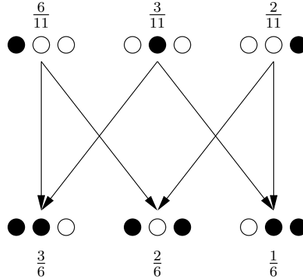
Figure 1: The case n = 4 and k = 2, 3 . Since B_1 is always 1, we omit it from the picture. For 2 \leq i \leq 4 , a filled circle in position i indicates that B_i^k = 1 ; an empty circle indicates that it is 0. The arrows indicate which states with k = 3 can be obtained from those with k = 2 ; the numbers are the probabilities p^k(b) of the states.
