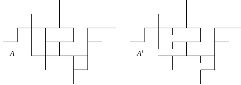
Figure 1: A lattice animal A and its associated cut-tree A^* .
