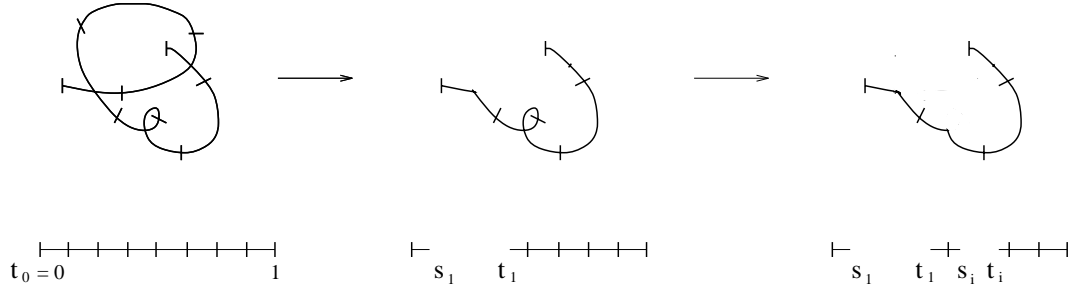
FIGURE 1. Construction of \gamma(t)
