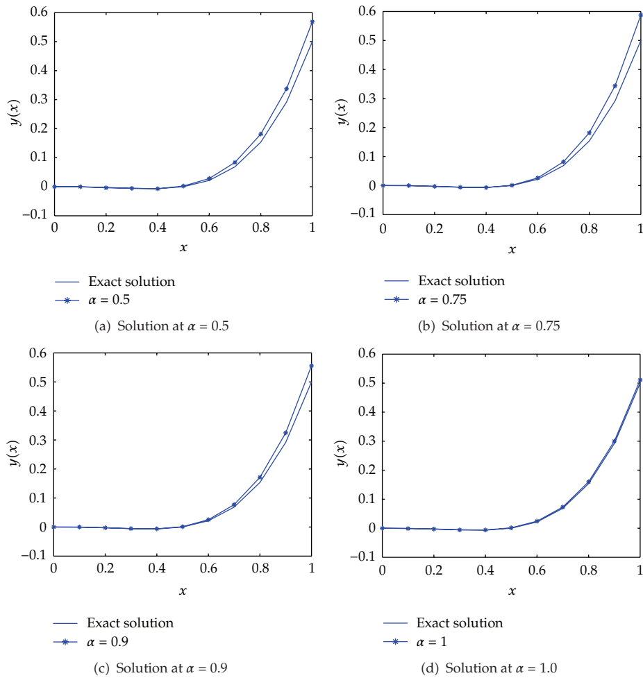
Figure 1: Approximate solutions for Example 3.1.
