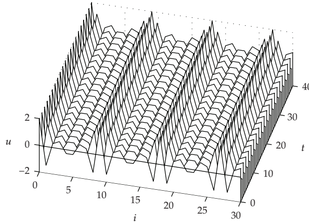
Figure 3: A (2, 9)-periodic traveling wave solution with velocity -27/4 .
