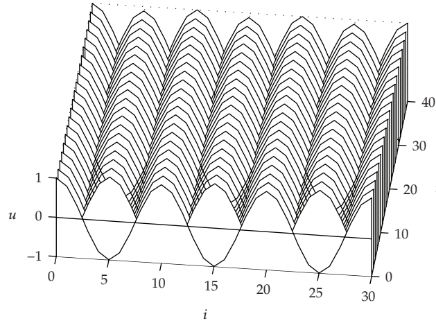
Figure 4: A (2, 10)-periodic traveling wave solution with velocity -15/7 .
