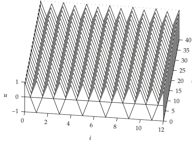
Figure 1: Doubly periodic traveling wave.
