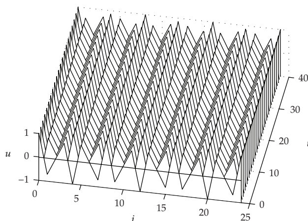
Figure 2: A (2, 8) -periodic traveling wave solution with velocity -4/5 .
