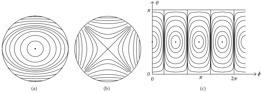
Figure 3: Counterrotating point vortices on a sphere with m = 2 viewed from (a) positive y -axis; (b) positive z -axis; (c) in \phi - \theta space.
