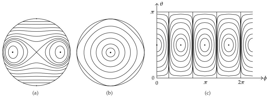
Figure 2: Corotating point vortices on a sphere with m = 4 viewed from (a) positive y -axis; (b) positive z -axis; (c) in \phi - \theta space.
