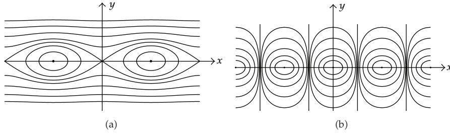
Figure 1: Point vortices on the plane: (a) a row of corotating vortices; (b) a row of counterrotating vortices.
