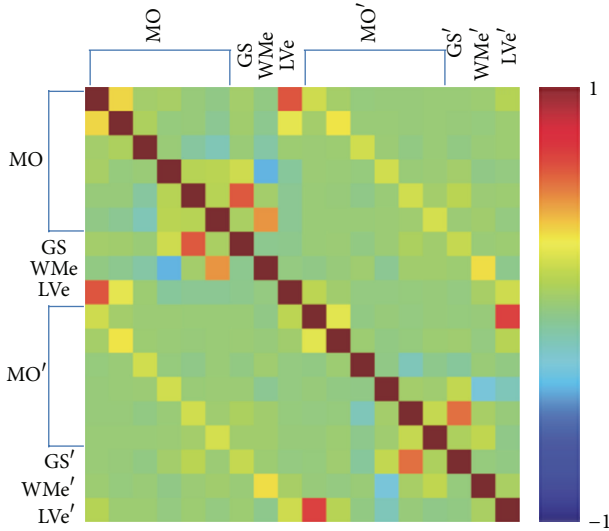
FIGURE 6: Cross-correlation matrix between the regressors. The correlation coefficients were averaged over all subjects ( N = 22 ). MO represents the six regressors containing rigid-body motion parameter estimates (three translations and three rotations). GS is the average RS-FMRI time series over all voxels in the brain mask. WMe and LVe refer to the RS-FMRI time series averaged within eroded white matter and eroded lateral ventricles, respectively. Prime marks ( ' ) indicate the first differences of the regressors. The regressors were obtained from the time series that were despiked, slice-timing corrected, and then volume registered, and spatial smoothing was not applied to avoid mixing signal across different brain-tissue masks.
