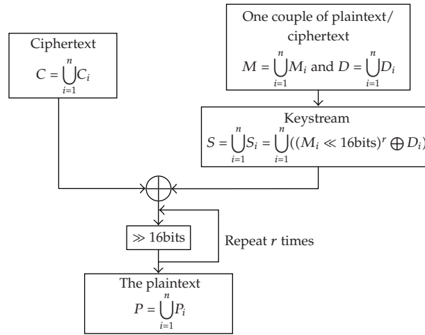
Figure 5: Flowchart of known plaintext attacks.
