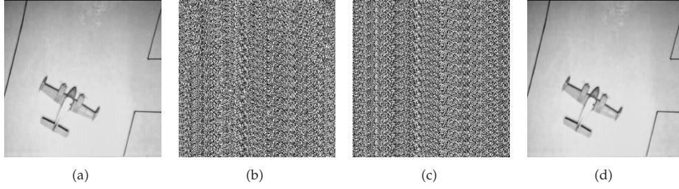
Figure 2: Results of the CPA: (a) the original image P ; (b) ciphered image C of P ; (c) ciphered image of M = 0000 ; (d) recovered image.
