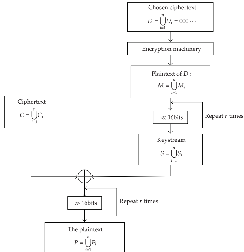
Figure 3: Flowchart of chosen ciphertext attacks.
