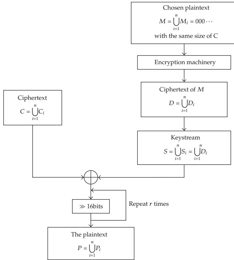
Figure 1: Flowchart of chosen plaintext attacks.
