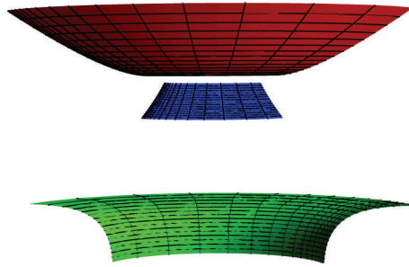
Figure 3: The hyperboloid S (blue) placed between its rational offsets S_{11} (green) and S_{12} (red).
