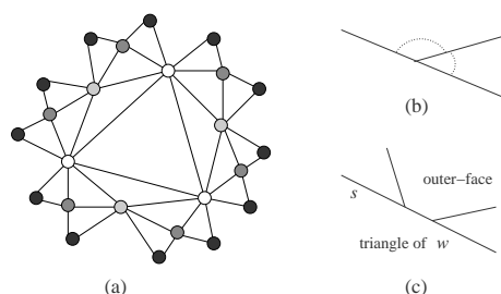
Figure 10: (a) The snowflake graph G_3 ; (b)–(c) illustration for the proof of Lemma 7.
