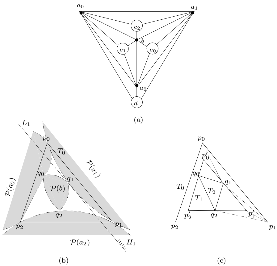
Figure 4: A graph G that does not have a proportional contact-representation with convex shapes.
