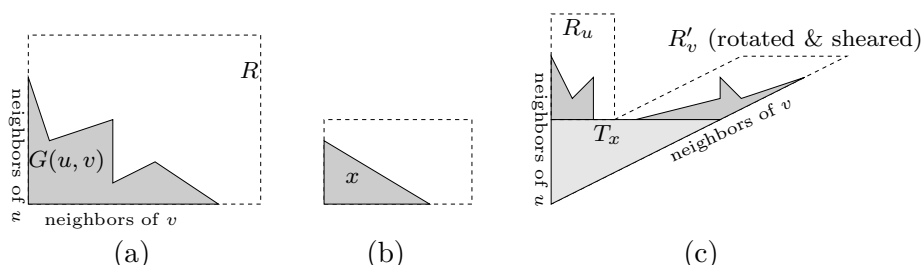
Figure 9: The construction for maximal outer-planar graphs: (a) requirements on drawing; (b) the base case; (c) combining the drawings.
