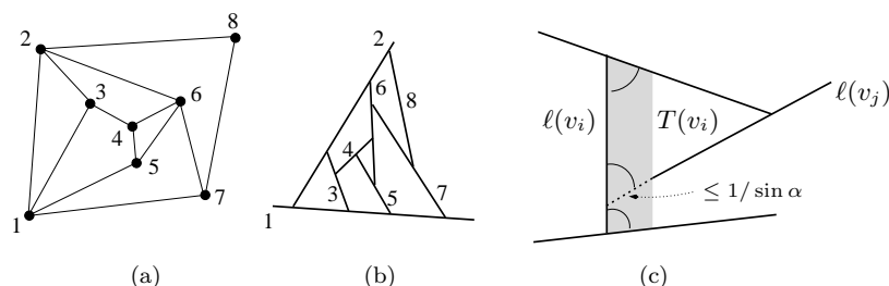
Figure 5: (a) A 2-segment graph; (b) a representation with line segments; the numbers indicate a suitable vertex order; (c) converting \ell(v_i) into a trapezoid T(v_i) and clipping \ell(v_j) . The indicated angles are all at least \alpha , hence the off-set is at most 1, and at most \frac{1}{\sin \alpha} is cut off \ell(v_j) .
