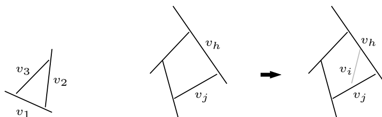
Figure 7: The 2-segment representation for 2-trees.
