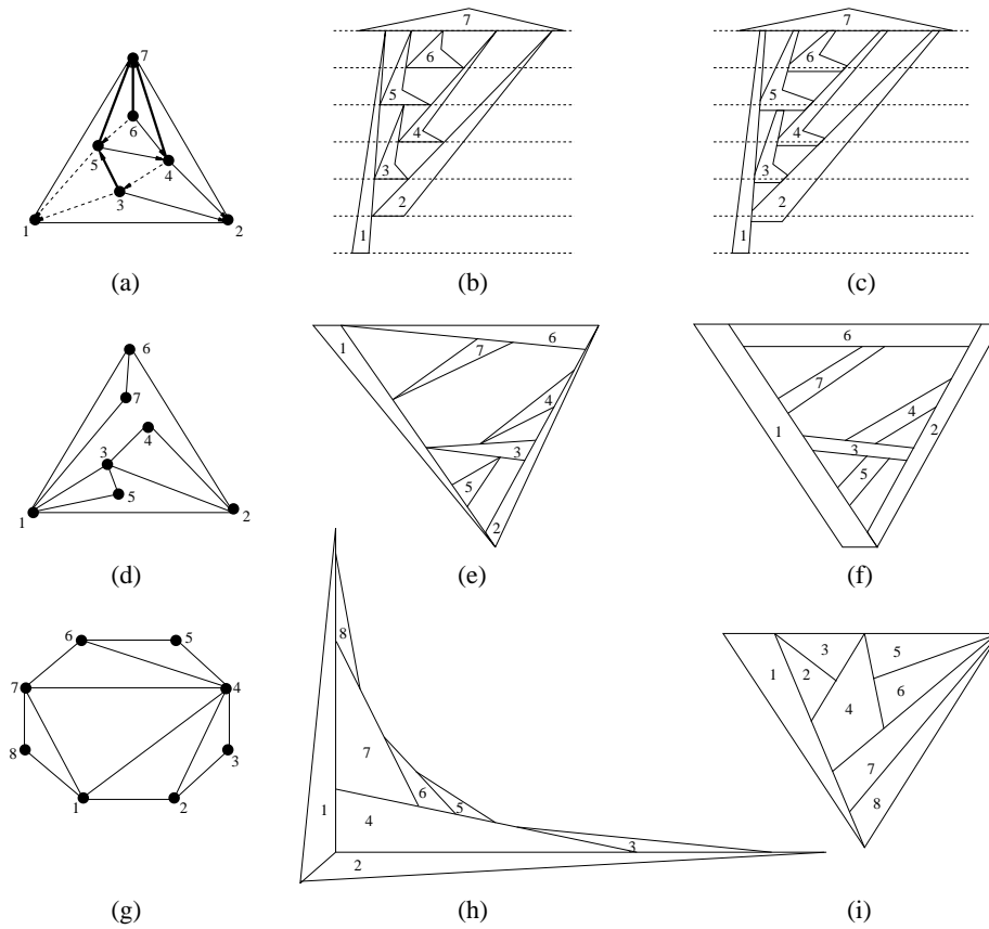
Figure 1: A general planar graph (a), its proportional point-contact representation with 4-sided non-convex polygons (b), and with its proportional side-contact representation with 7-sided polygons (c). A 2-tree (d), its proportional point-contact representation with triangles (e), and its proportional side-contact representation with trapezoids (f). A maximal outer-planar graph (g), its hole-free proportional side-contact representations with triangles (h), and with 4-sided convex polygons (i).
