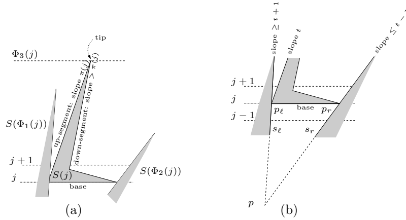
Figure 3: (a) Adding j ; (b) computing the width of the base.
