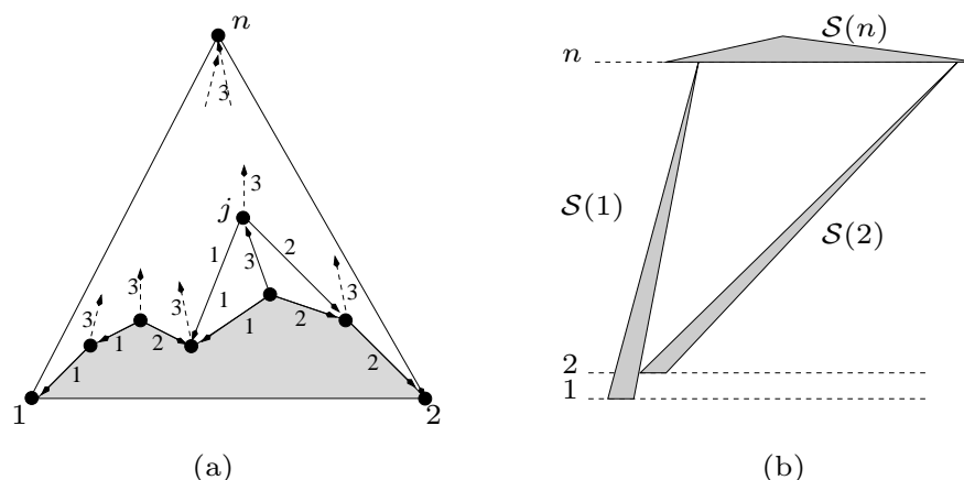
Figure 2: (a) The canonical order and T_i (marked by labels); (b) the placement of 1, 2, n .
