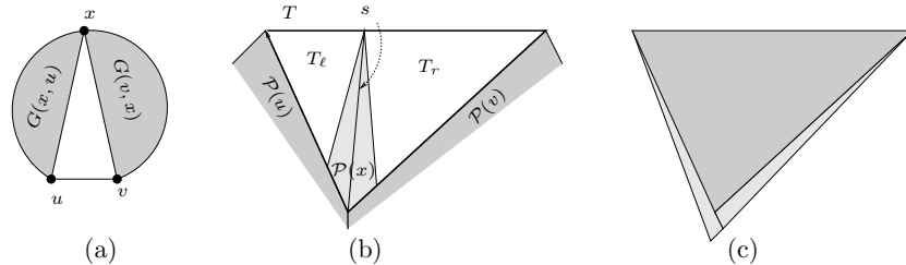
Figure 8: The construction for maximal outer-planar graphs: (a) the graph; (b) splitting triangle T suitably; (c) adding u and v in the outer-most recursion.
