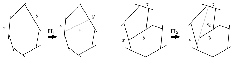
Figure 6: The addition of segment s_i .
