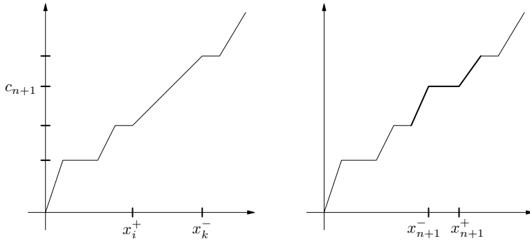
Figure 3: Inserting the stop value c_{n+1}
