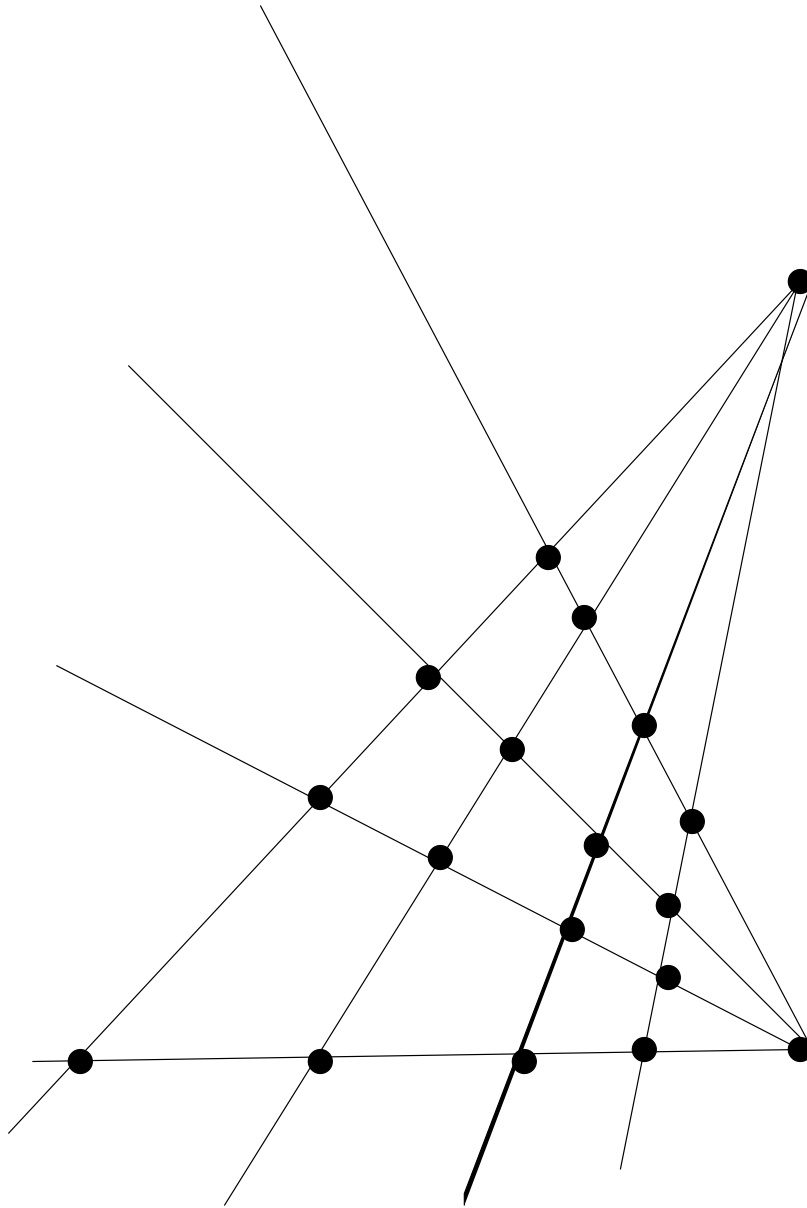
FIGURE 4. A Furstenburg set when viewed from x_1 and x'_1 . Note how this resembles a projective transformation of Figure 3.
