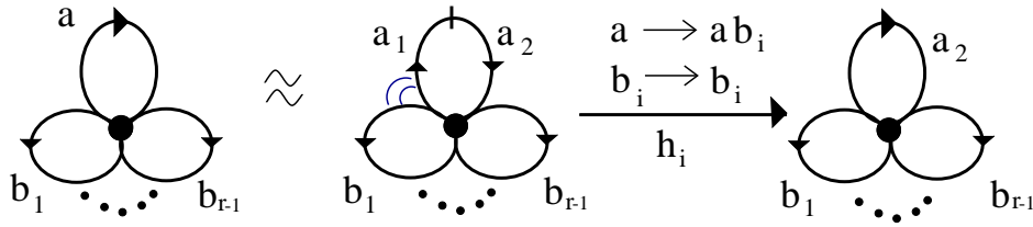
FIGURE 4. Proper full fold.
