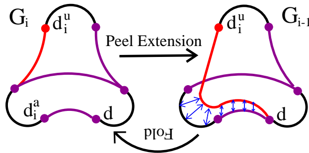
FIGURE 7. Peel Extension: Note that the first, second, and third edges of the peel concatenate to form the red edge [d_i^u, d] in G_{i-1} and that copies of [\overline{d_i^a}, d_i^a] and [d_i^a, d] remain in G_{i-1} .
