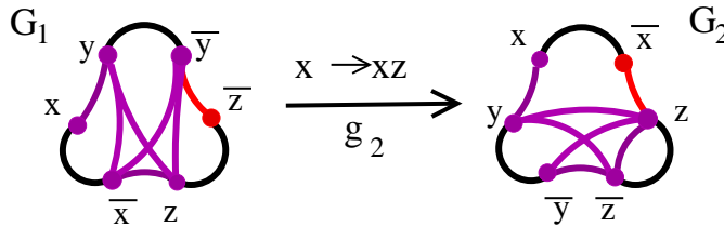
FIGURE 6. The induced map for g_2 : x \mapsto xz sends vertex \bar{x} of G_1 to vertex \bar{z} of G_2 and every other vertex of G_1 to the identically labeled vertex of G_2 . [y] in G_1 maps to [y] in G_2 , [z] in G_1 maps to [z] in G_2 , and [x] in G_1 maps to [x] \cup [\bar{x}, z] \cup [z] in G_2 . The purple edge [\bar{x}, y] in G_1 maps to the purple edge [\bar{z}, y] in G_2 , the purple edge [\bar{x}, \bar{y}] in G_1 maps to the purple edge [\bar{z}, \bar{y}] in G_2 , [\bar{x}, z] in G_1 maps to the purple edge [\bar{z}, z] in G_2 , and each other purple edge in G_1 is sent to the identically labeled purple edge in G_2 . The red edge [\bar{z}, \bar{y}] in G_1 maps to the purple edge [\bar{z}, \bar{y}] in G_2 .
