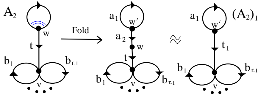
FIGURE 1. a_1 is the portion of a not folded, a_2 is the edge created by the fold, w' is the vertex created by the fold, and t_1 is a_2 \cup t without the (now unnecessary) vertex w .
