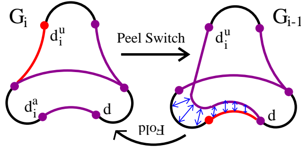
FIGURE 8. Peel Switch (when d_i^a only belongs to one purple edge in G_{i-1} ): The first, second, and third edges of the peel concatenate to form a purple edge [d_i^u, d] in G_{i-1} . The determining edge [d_i^a, d] is the red edge of G_{i-1} , with red vertex d_i^a .
