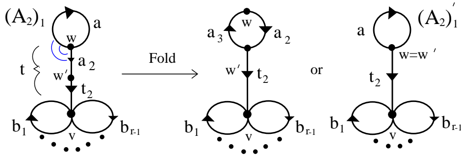
FIGURE 2. Of the two scenarios on the right, the leftmost is where the fold ends in the middle of a . a_2 is a possible portion of a folded with the portion of t , a_3 would be the portion of a not folded with t , and t_2 would be the portion of t not folded with a .
