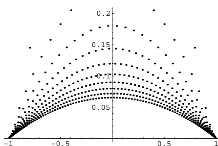
FIGURE 1. Zero distribution of \pi_n , n = 10(10)100 , for \lambda = 11 and \zeta \approx 14.47550068655454123845163765541315197630481 (a zero of J_{10} )
