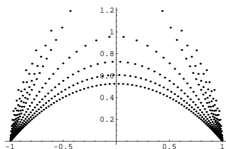
FIGURE 2. Zero distribution of \pi_n , n = 10(10)100 , for \lambda = 11 and \zeta \approx 100.71634047409274068436610723206019123535653 (a zero of J_{10} )
