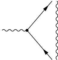
Figure 4. A degenerate but disconnected process.
