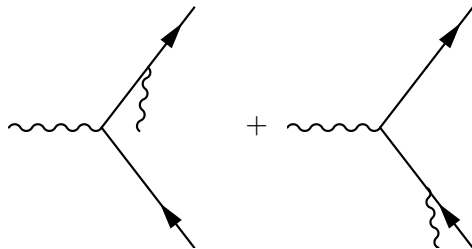
Figure 2. Soft photon absorption from the in-coming and out-going electron.
