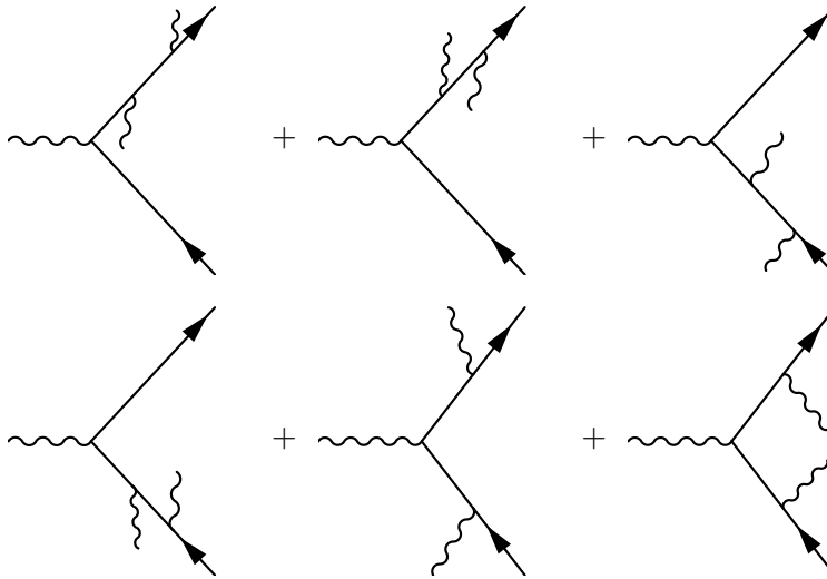
Figure 3. Soft photon emission and absorption from the in-coming and out-going electron.
