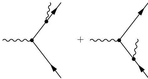
Figure 1. Soft photon emission from the in-coming and out-going electron.
