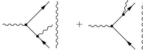
Figure 5. A degenerate initial state photon and two final state photons.
