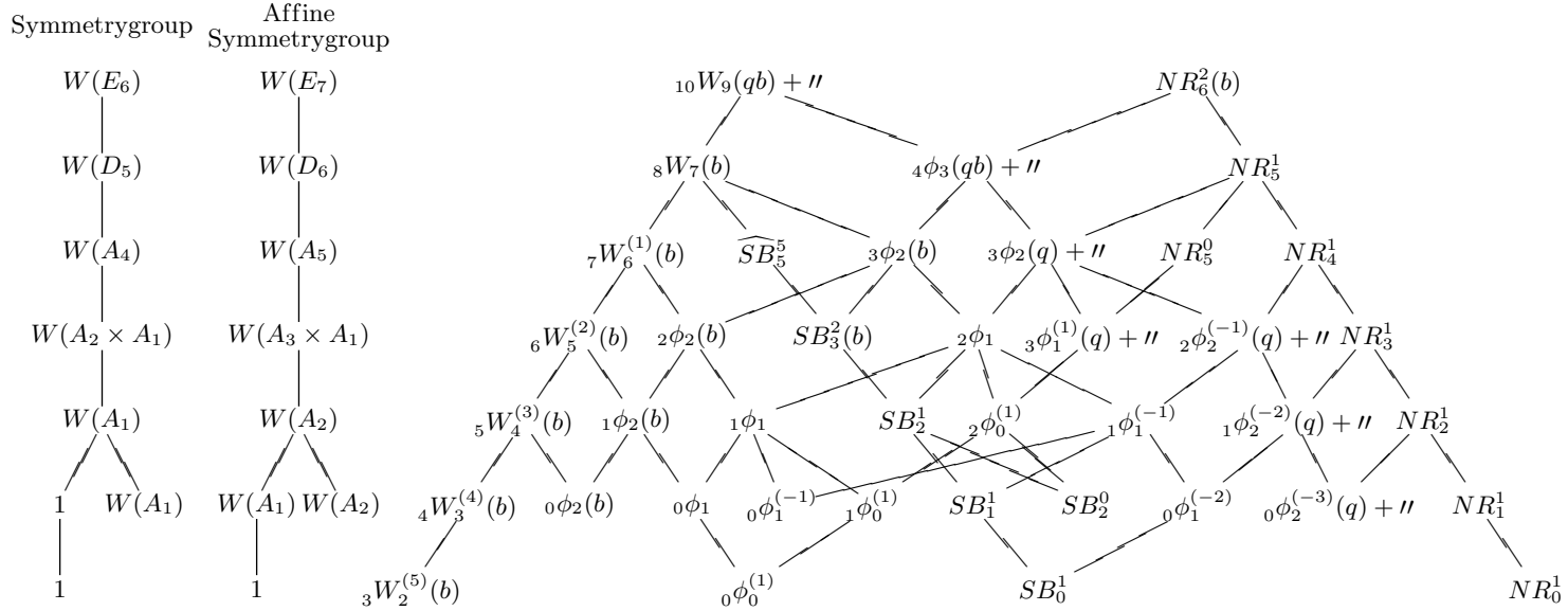
Figure 2. The simplicial faces of P^{(1)} .
