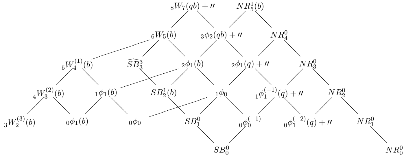
Figure 3. The simplicial faces of P_I^{(0)} , P_{II}^{(0)} and P_{III}^{(0)} .
