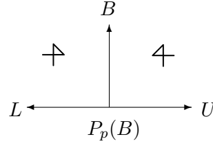
Figure 3. Triangular diagram relating the subalgebras L , U and B . P_p(B) is a polynomial of the p th degree in B generators. It is a generalization of the Gauss decomposition for semi-simple algebras where p = 1 .
