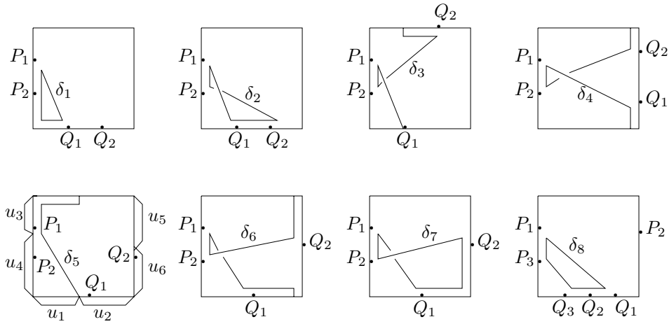
Figure 9: Constructing curve \delta
