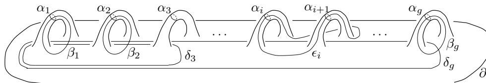
Figure 1: Surface S_{g,1}
