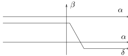
Figure 4: Curve \delta has smaller intersection with \alpha and \beta .
