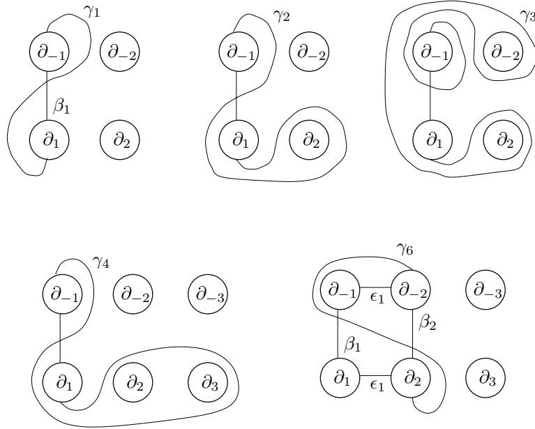
Figure 15: Curves \gamma_i
