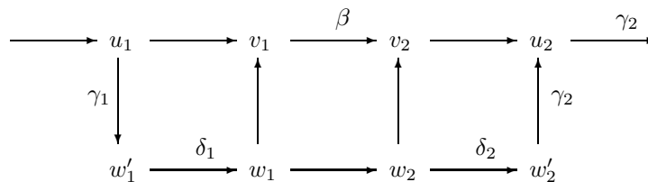
Figure 10: Reducing a path of radius m
