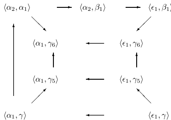
Figure 17: Reduction for paths of type (C5)
