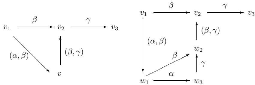
Figure 7: Path of radius 0, Case 2
