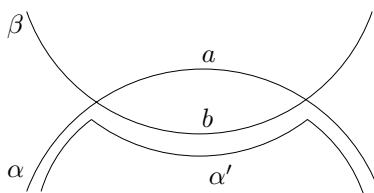
Figure 3: Curves \alpha and \beta form a 2-gon.
