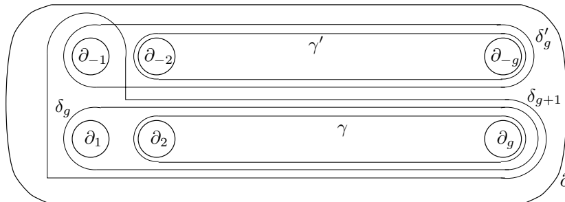
Figure 18: Spin maps in the proof of Theorem 3
