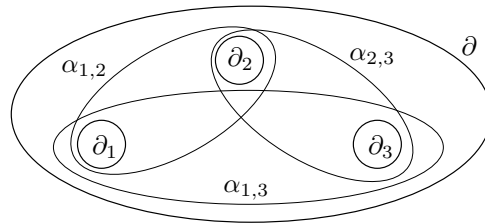
Figure 11: Lantern relation
