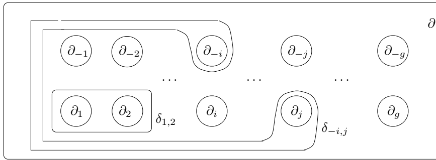
Figure 13: Curves \delta_{i,j} on S_0
