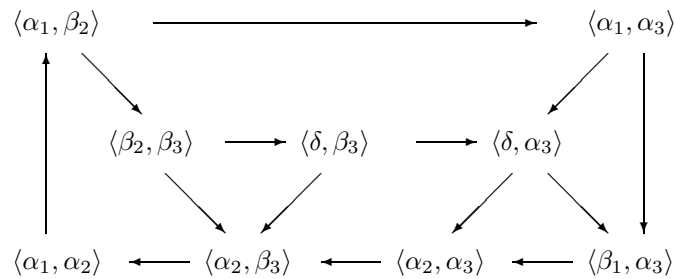
Figure 5: Hexagonal path
