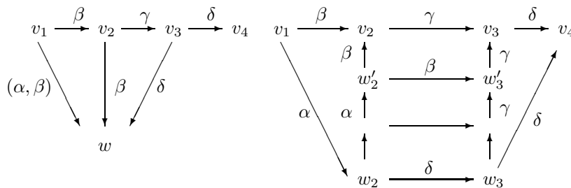
Figure 8: Path of radius 0, Case 3
