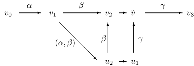
Figure 6: Path of radius 0, Case 1
