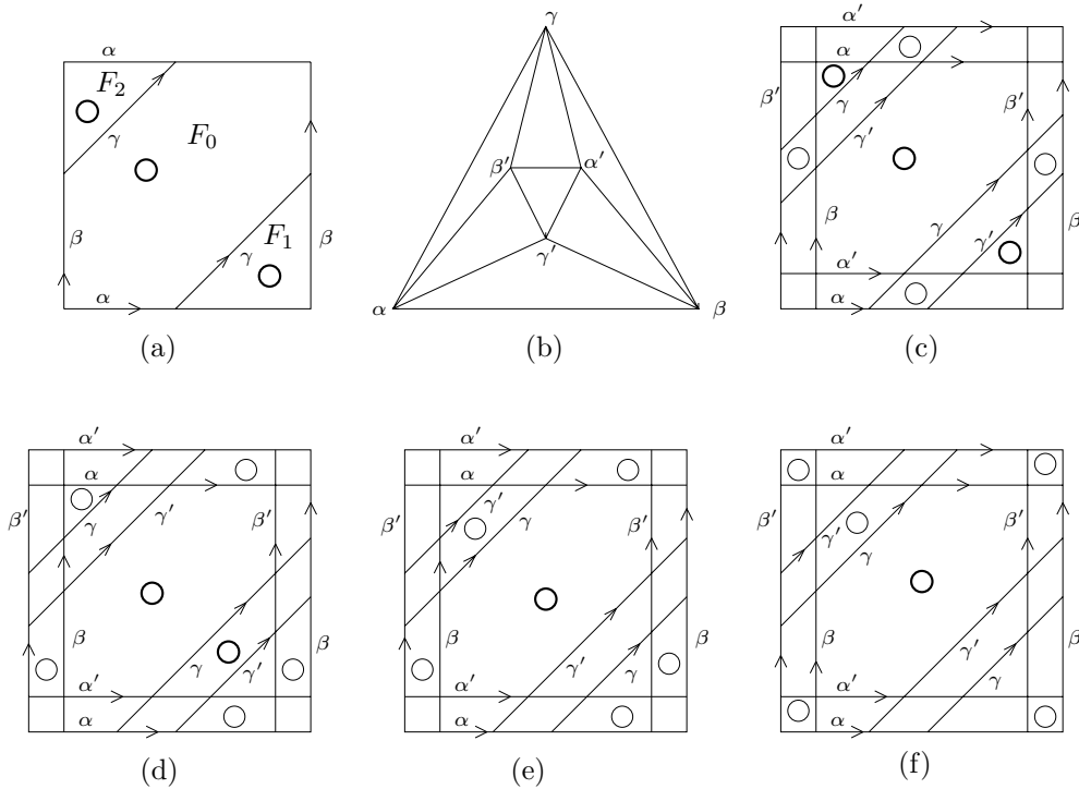
Figure 16: Reduction for paths of type (C3)
