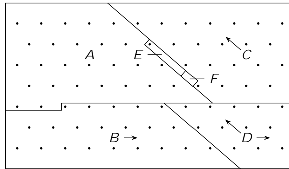
Figure 6: Tightening the hexagonal circle packing
