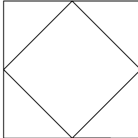
Figure 28: \tilde{G} contains a square
