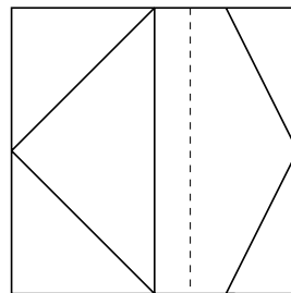
Figure 26: \tilde{G} contains a triangle (dashed arc included along with \tilde{G} to indicate that a bicoloring, as required, is possible)
