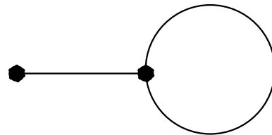
Figure 9: The graph on which M is modelled
