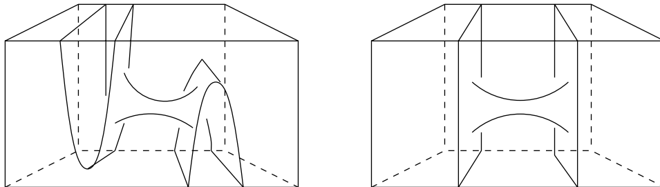
Figure 25: Two isotopic possibilities
