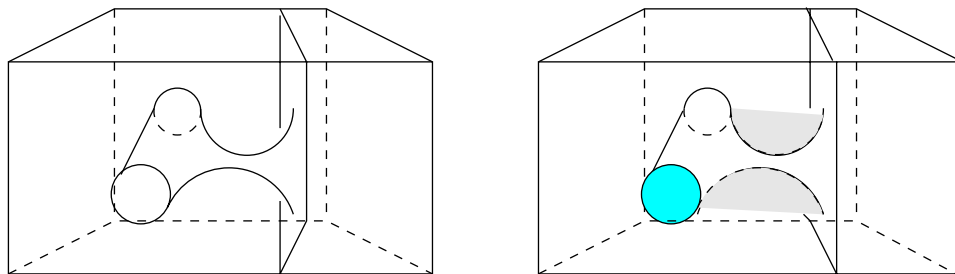
Figure 24: Another stabilized possibility
