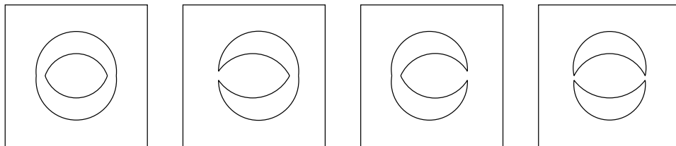
Figure 18: The regions North, East, West and South
