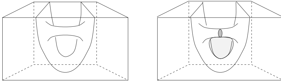
Figure 23: Compressible component meets annulus parallel into T_{t_0 \pm \epsilon}
