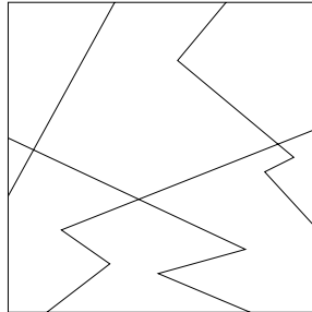
Figure 15: The Rubinstein–Scharlemann graph
