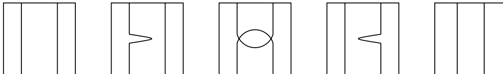
Figure 22: Adding a 1–handle
