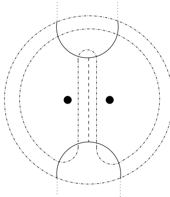
Figure 12: The active component is an edge manifold
