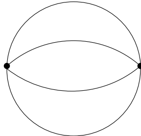
Figure 17: \tilde{G} is contractible
