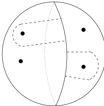
Figure 5: Schematic for Heegaard splitting after amalgamation
