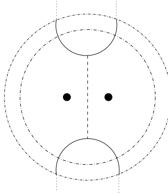
Figure 11: The active component is a vertex manifold
