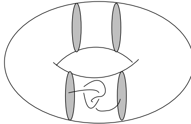
Figure 13: Schematic for a Heegaard splitting intersecting a solid torus
