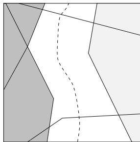
Figure 19: A monotone path through unlabelled regions
