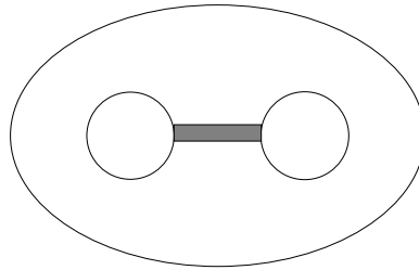
Figure 7: Schematic for Heegaard splitting of a graph manifold
