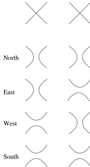
Figure 16: How S_s meets T_t in the four regions North, East, West and South meeting (s_0, t_0)
