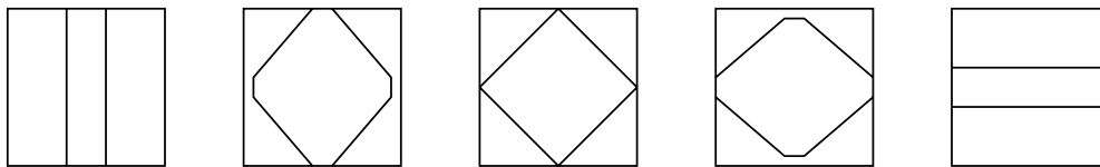
Figure 29: Another way of adding a 1-handle
