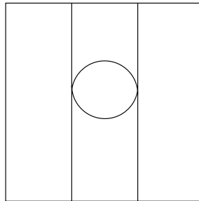
Figure 21: \tilde{G} contains a bigon
