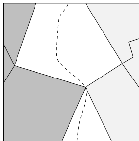
Figure 20: A monotone path through unlabelled regions
