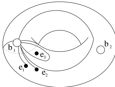
Figure 3: Schematic for a vertical Heegaard splitting of a Seifert fibered space
