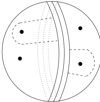
Figure 4: Schematic for a generalized strongly irreducible Heegaard splitting
