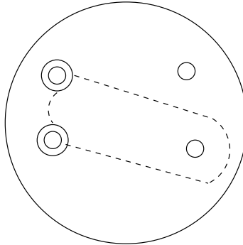
Figure 10: Schematic for vertical Heegaard splittings of graph manifold with boundary
