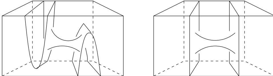
Figure 14: Two isotopic possibilities
