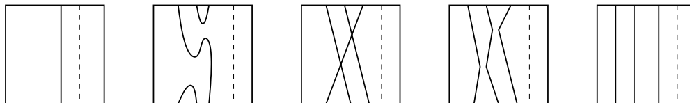
Figure 27: Adding an “essential” 1–handle
