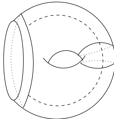
Figure 8: Schematic for Heegaard splitting of a graph manifold
